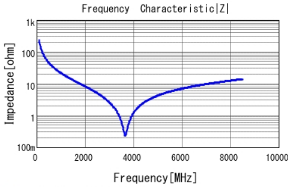
■ GJM0335C1E6R8BB01 |Z| DCOV, 25degC
