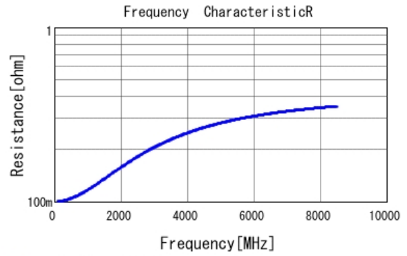
■ GJM0335C1E6R8BB01 R DCOV, 25degC
