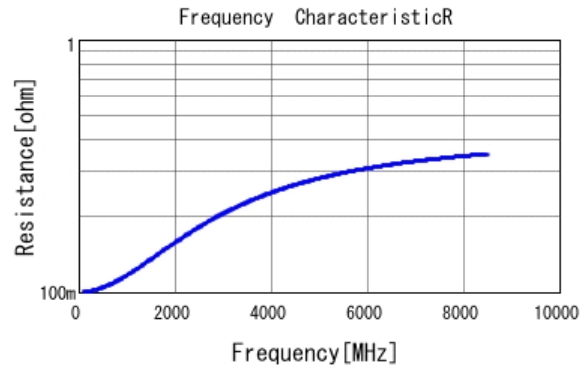
■ GJM0335C1E6R8CB01 R DCOV, 25degC
