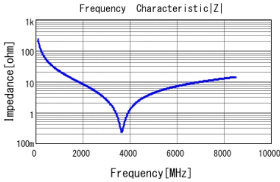
■ GJM0335C1E6R8CB01 |Z| DCOV, 25degC
