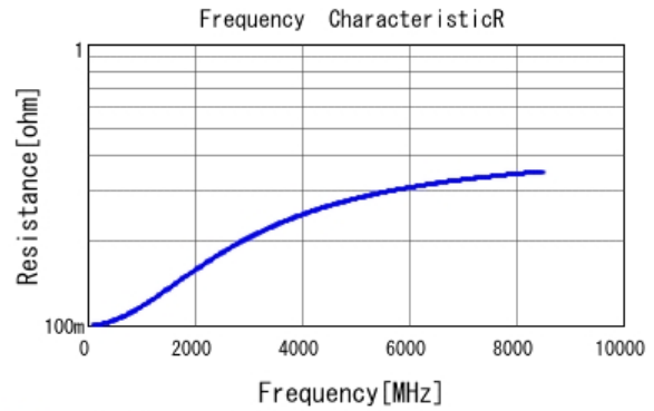
■ GJM0335C1E6R8WB01 R DCOV, 25degC
