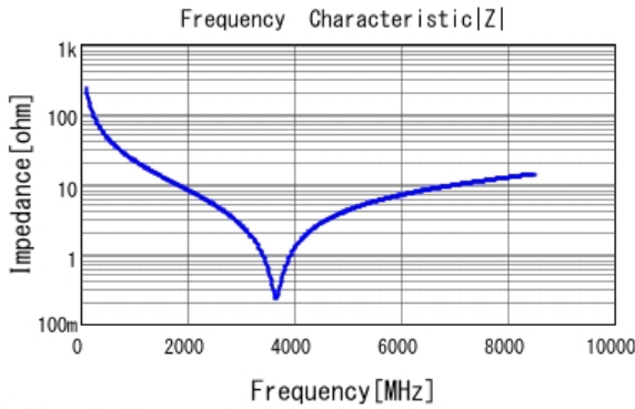
■ GJM0335C1E6R8WB01 |Z| DCOV, 25degC
