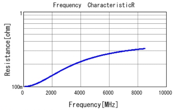
■ GJM0335C1E8R0BB01 R DCOV, 25degC
