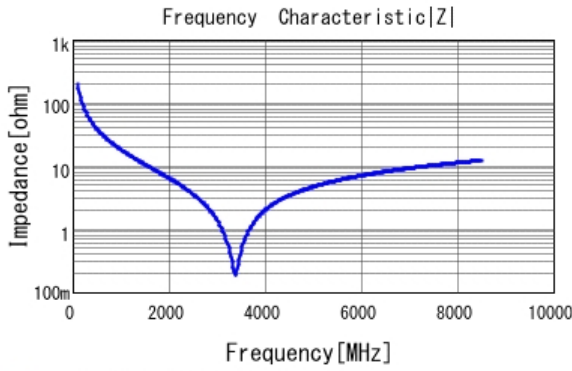
■ GJM0335C1E8R0BB01 |Z| DCOV, 25degC
