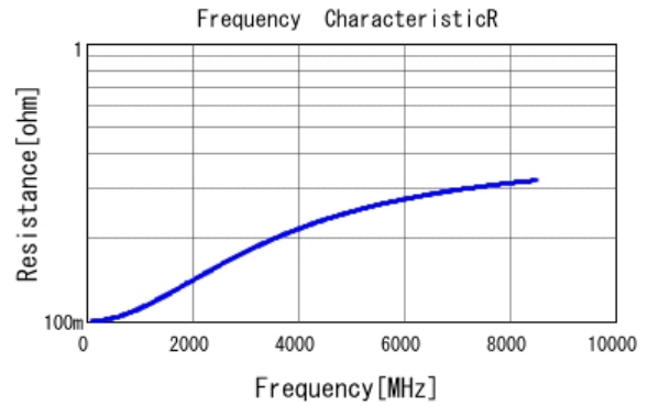
■ GJM0335C1E8R2CB01 R DCOV, 25degC
