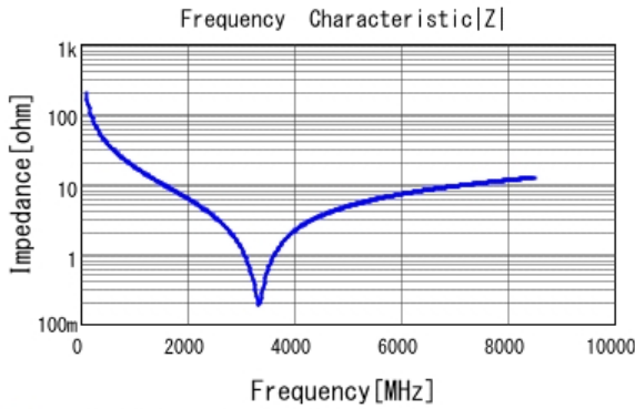
■ GJM0335C1E8R2CB01 |Z| DCOV, 25degC
