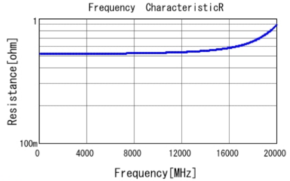
■ GJM0335C1ER30WB01 R DCOV, 25degC
