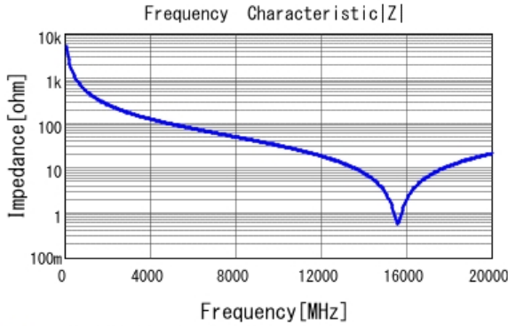
■ GJM0335C1ER30WB01 |Z| DCOV, 25degC
