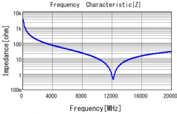
■ GJM0335C1ER50BB01 |Z| DC0V, 25degC
