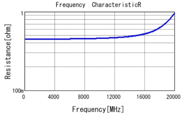
■ GJM0335C1ER50BB01 R DC0V, 25degC
