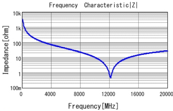
■ GJM0335C1ER50WB01 |Z| DC0V, 25degC
