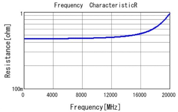
■ GJM0335C1ER50WB01 R DC0V, 25degC
