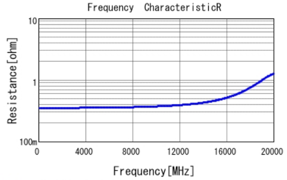
■ GJM0335C1ER80BB01 R DC0V, 25degC
