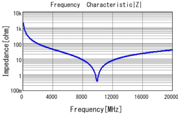
■ GJM0335C1ER80BB01 |Z| DC0V, 25degC
