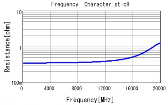
■ GJM0335C1ER80WB01 R DCOV, 25degC
