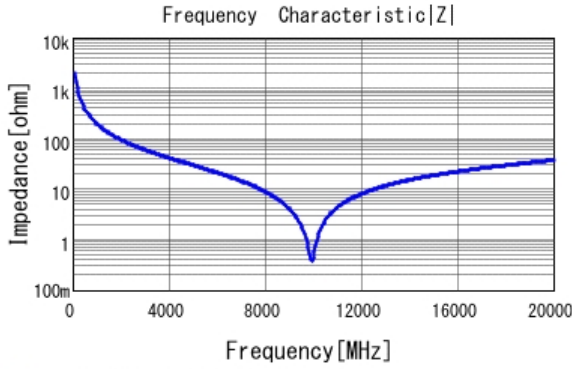
■ GJM0335C1ER80WB01 |Z| DCOV, 25degC
