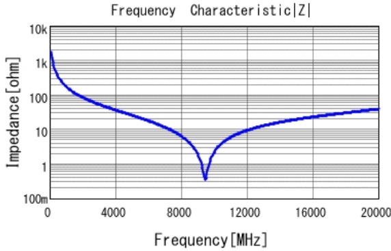
■ GJM0335C1ER90WB01 |Z| DC0V, 25degC
