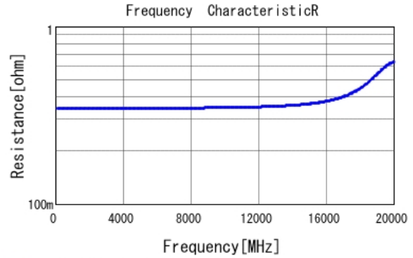
■ GJM0335C1ER90WB01 R DC0V, 25degC
