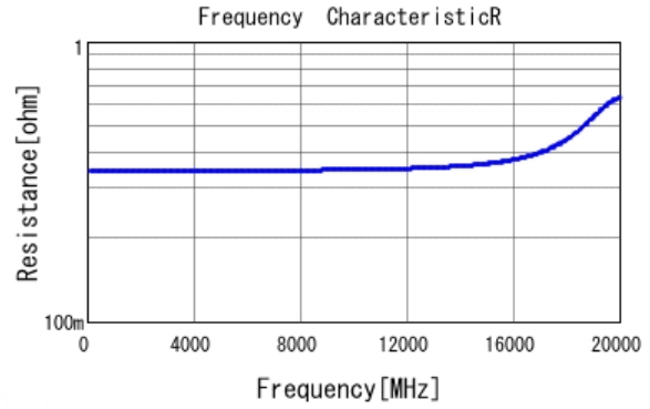
■ GJM0335C1HR90WB01 R DCOV, 25degC
