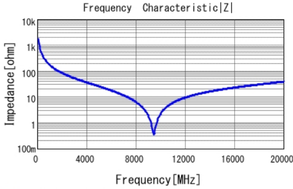
■ GJM0335C1HR90WB01 |Z| DCOV, 25degC
