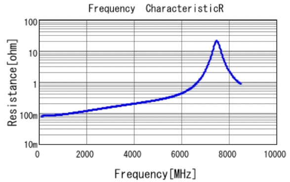
■ GJM1552C1H9R0CB01 R DCOV, 20degC
