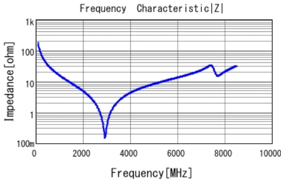
■ GJM1552C1H9R0CB01 |Z| DCOV, 20degC
