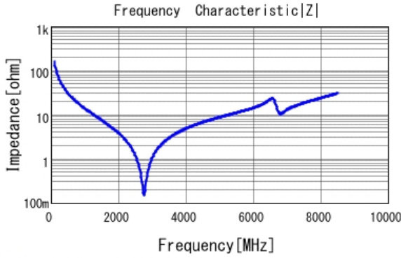
■ GJM1555C1H100GB01 |Z| DCOV, 25degC
