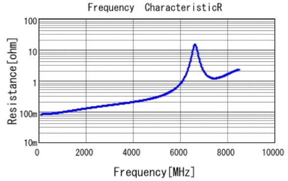
■ GJM1555C1H100GB01 R DCOV, 25degC
