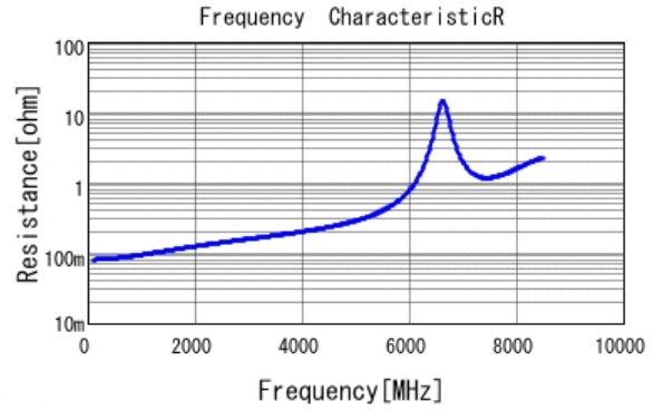
■ GJM1555C1H100JB01 R DCOV, 25degC
