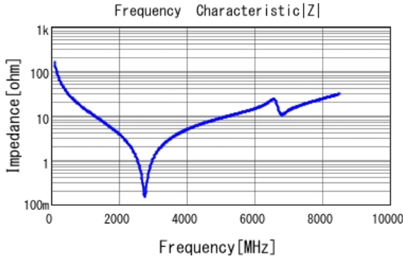
■ GJM1555C1H100JB01 |Z| DCOV, 25degC
