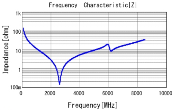
■ GJM1555C1H120JB01 |Z| DCOV, 25degC
