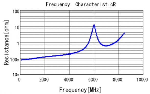
■ GJM1555C1H120JB01 R DCOV, 25degC
