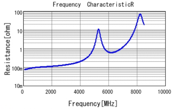
■ GJM1555C1H160GB01 R DCOV, 25degC
