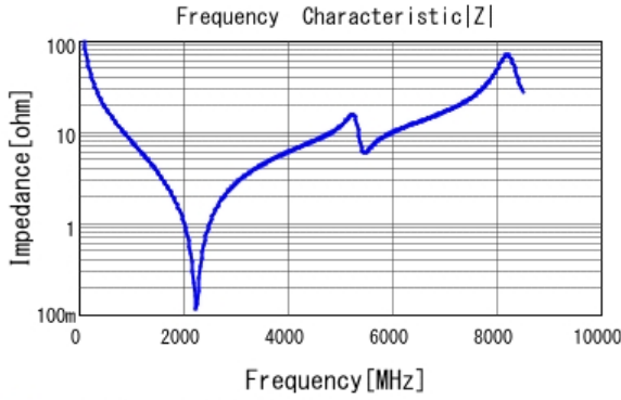
■ GJM1555C1H160GB01 |Z| DCOV, 25degC
