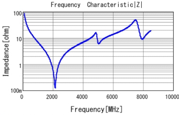
■ GJM1555C1H180FB01 |Z| DCOV, 25degC
