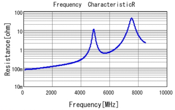
■ GJM1555C1H180FB01 R DCOV, 25degC
