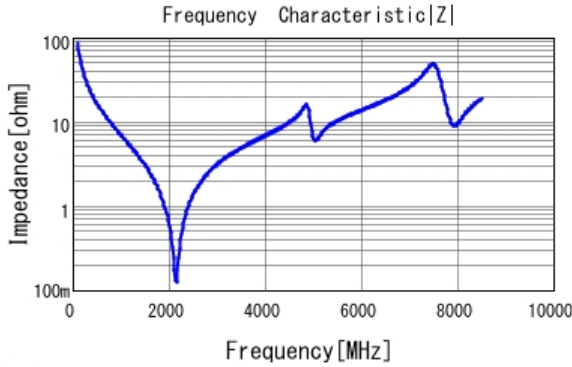
■ GJM1555C1H180GB01 |Z| DCOV, 25degC
