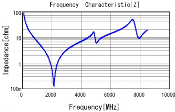
■ GJM1555C1H180JB01 |Z| DCOV, 25degC
