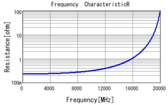
■ GJM1555C1H1R0BB01 R DC0V, 25degC
