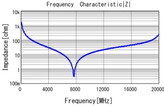
■ GJM1555C1H1R0BB01 |Z| DC0V, 25degC
