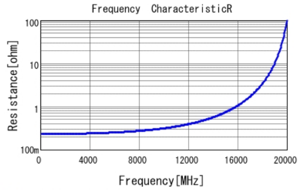
■ GJM1555C1H1R0CB01 R DC0V, 25degC
