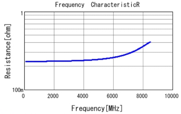
■ GJM1555C1H1R1CB01 R DCOV, 25degC
