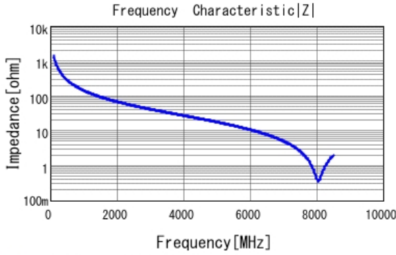
■ GJM1555C1H1R1CB01 |Z| DCOV, 25degC
