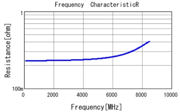
■ GJM1555C1H1R1WB01 R DCOV, 25degC
