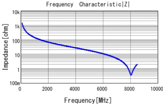
■ GJM1555C1H1R1WB01 |Z| DCOV, 25degC
