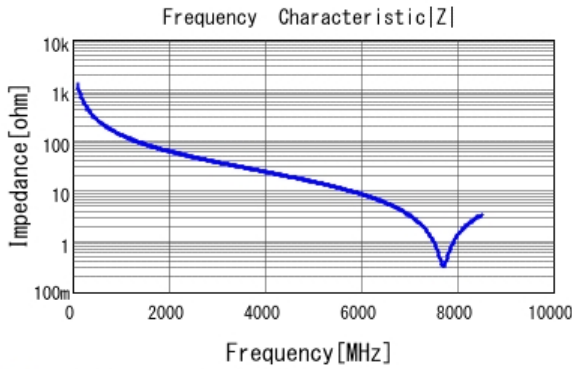
■ GJM1555C1H1R2CB01 |Z| DC0V, 25degC
