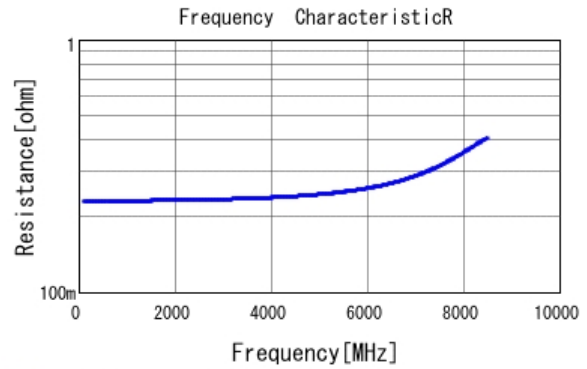
■ GJM1555C1H1R2CB01 R DC0V, 25degC
