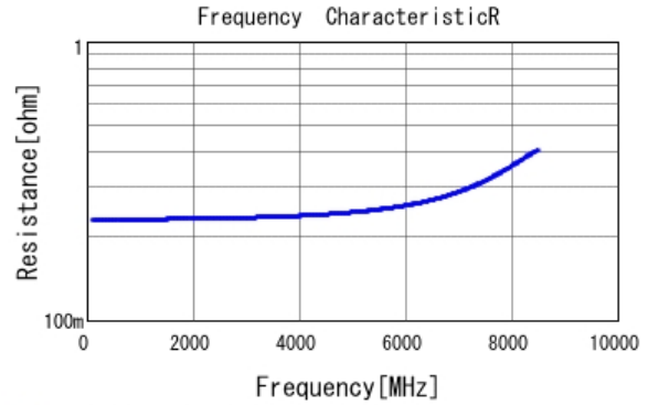
■ GJM1555C1H1R3WB01 R DCOV, 25degC
