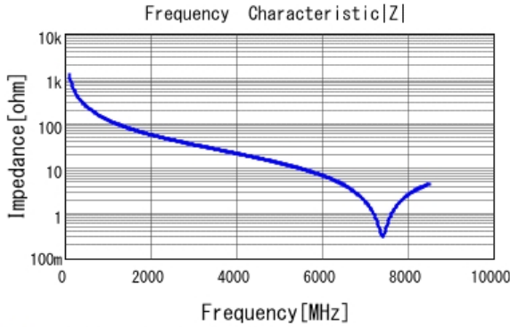
■ GJM1555C1H1R3WB01 |Z| DCOV, 25degC
