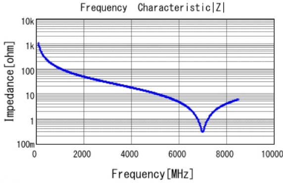
■ GJM1555C1H1R5BB01 |Z| DC0V, 25degC
