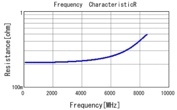
■ GJM1555C1H1R5CB01 R DC0V, 25degC
