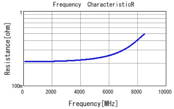
■ GJM1555C1H1R5WB01 R DCOV, 25degC
