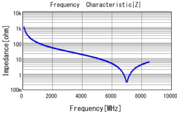
■ GJM1555C1H1R5WB01 |Z| DCOV, 25degC
