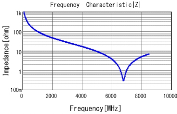
■ GJM1555C1H1R6BB01 |Z| DCOV, 25degC
