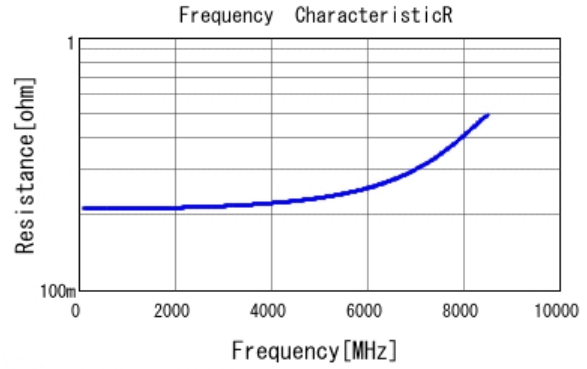
■ GJM1555C1H1R6BB01 R DCOV, 25degC
