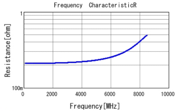
■ GJM1555C1H1R6CB01 R DC0V, 25degC
