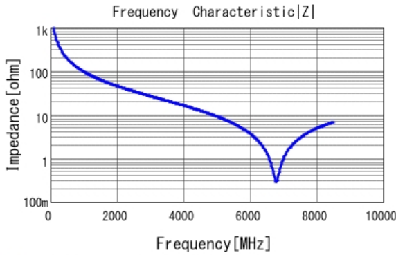
■ GJM1555C1H1R6CB01 |Z| DC0V, 25degC
