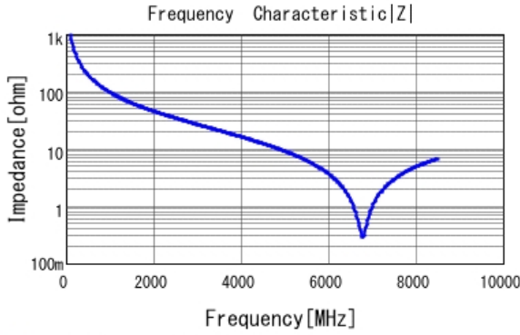
■ GJM1555C1H1R6WB01 |Z| DCOV, 25degC
