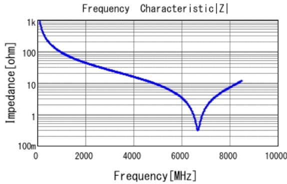
■ GJM1555C1H1R7BB01 |Z| DC0V, 25degC
