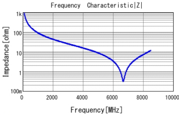
■ GJM1555C1H1R7WB01 |Z| DCOV, 25degC
