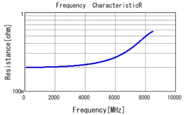
■ GJM1555C1H1R7WB01 R DCOV, 25degC
