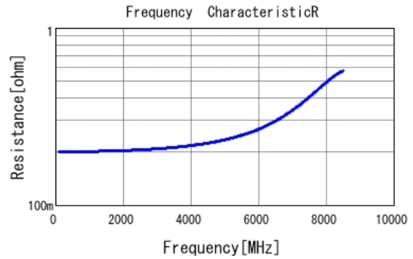
■ GJM1555C1H1R8BB01 R DC0V, 25degC
