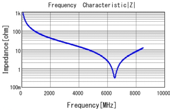
■ GJM1555C1H1R8BB01 |Z| DC0V, 25degC
