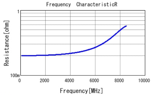
■ GJM1555C1H1R8CB01 R DCOV, 25degC
