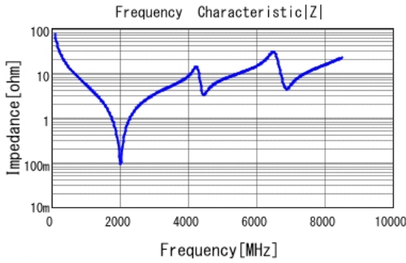
■ GJM1555C1H220JB01 |Z| DC0V, 25degC
