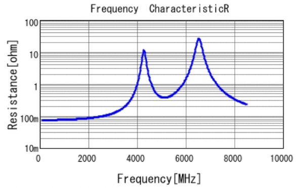
■ GJM1555C1H220JB01 R DC0V, 25degC
