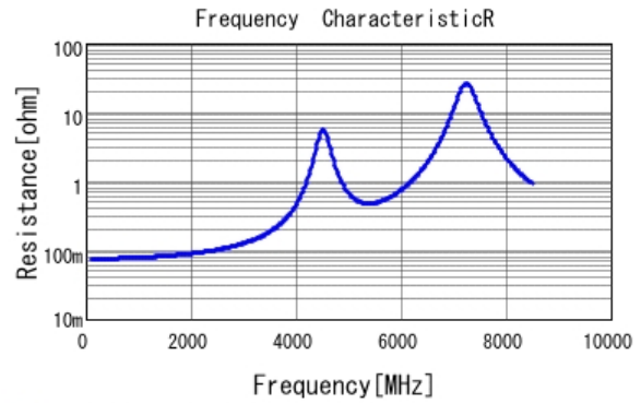
■ GJM1555C1H240FB01 R DC0V, 25degC
