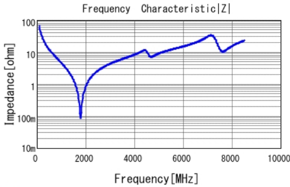
■ GJM1555C1H240FB01 |Z| DC0V, 25degC
