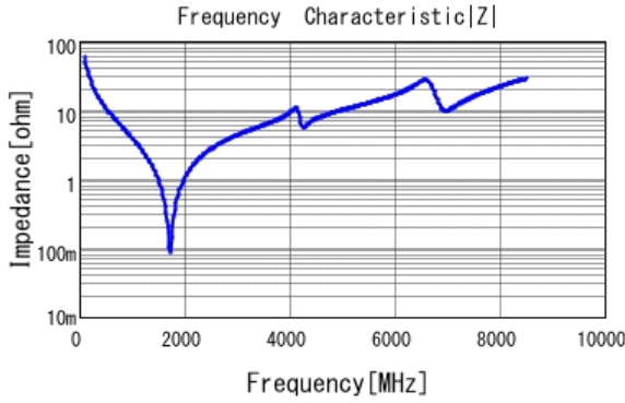
■ GJM1555C1H270JB01 |Z| DC0V, 25degC
