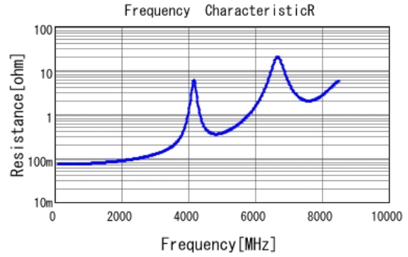
■ GJM1555C1H270JB01 R DC0V, 25degC
