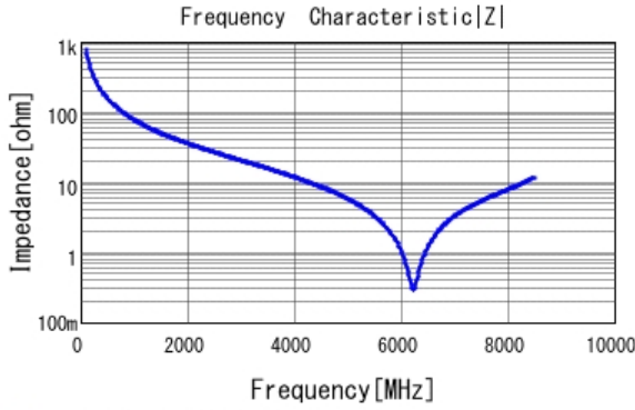
■ GJM1555C1H2R0BB01 |Z| DCOV, 25degC
