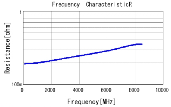
■ GJM1555C1H2R0BB01 R DCOV, 25degC
