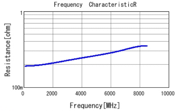
■ GJM1555C1H2R0CB01 R DCOV, 25degC
