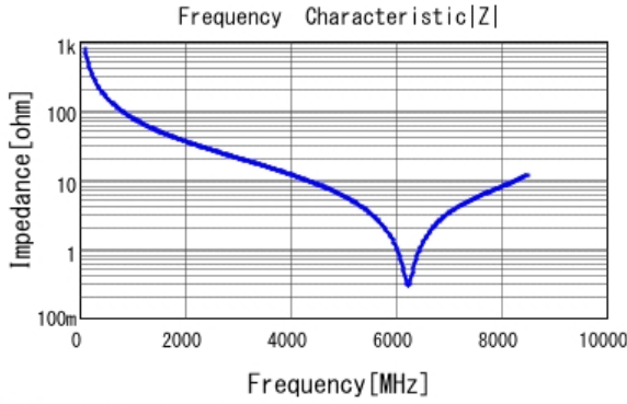
■ GJM1555C1H2R0CB01 |Z| DCOV, 25degC
