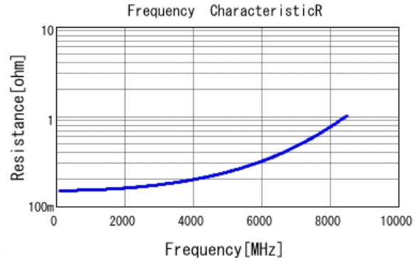
■ GJM1555C1H2R4WB01 R DC0V, 25degC
