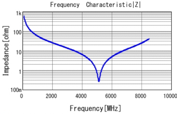
■ GJM1555C1H2R7BB01 |Z| DC0V, 25degC
