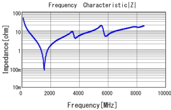
■ GJM1555C1H330GB01 |Z| DC0V, 25degC
