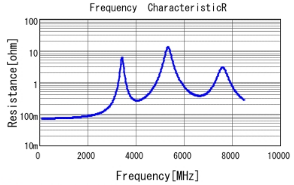
■ GJM1555C1H360FB01 R DC0V, 25degC
