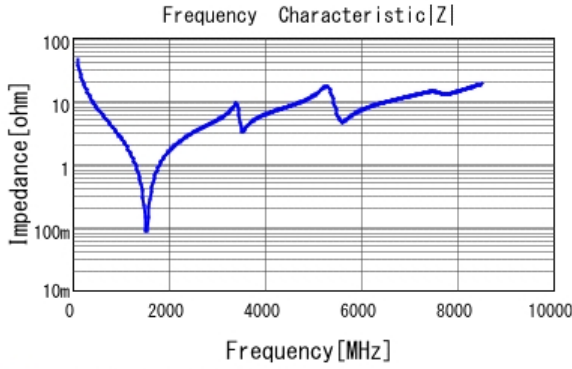
■ GJM1555C1H360FB01 |Z| DC0V, 25degC
