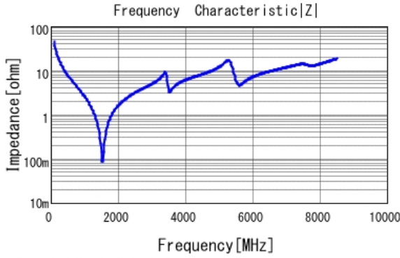
■ GJM1555C1H360JB01 |Z| DC0V, 25degC
