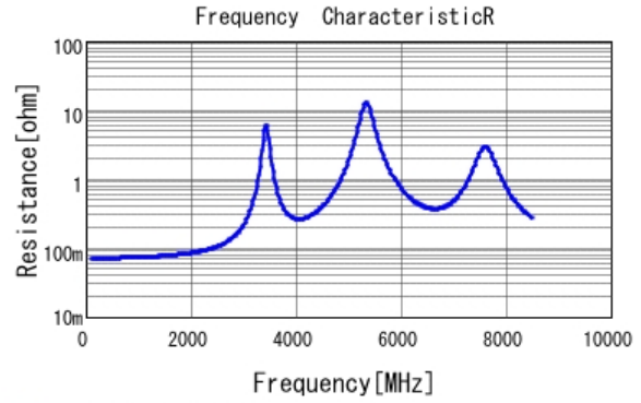
■ GJM1555C1H360JB01 R DC0V, 25degC
