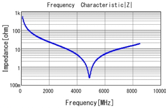
■ GJM1555C1H3R0BB01 |Z| DC0V, 25degC
