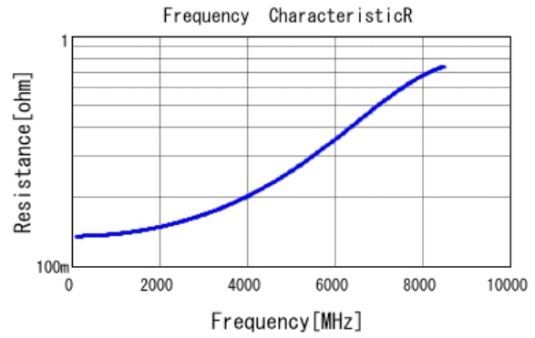
■ GJM1555C1H3R0BB01 R DC0V, 25degC
