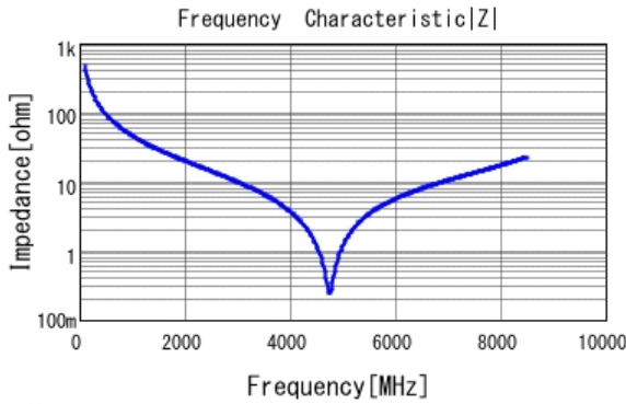
■ GJM1555C1H3R3CB01 |Z| DCOV, 25degC
