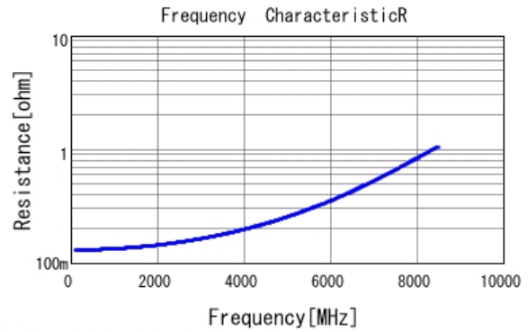
■ GJM1555C1H3R3CB01 R DCOV, 25degC
