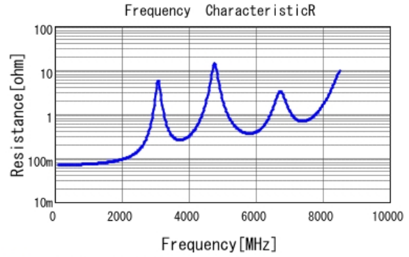
■ GJM1555C1H430FB01 R DC0V, 25degC
