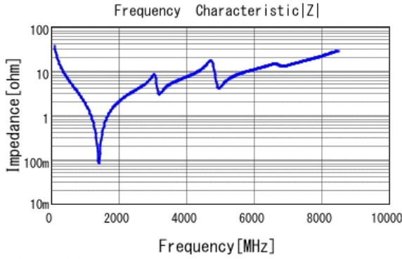
■ GJM1555C1H430FB01 |Z| DC0V, 25degC
