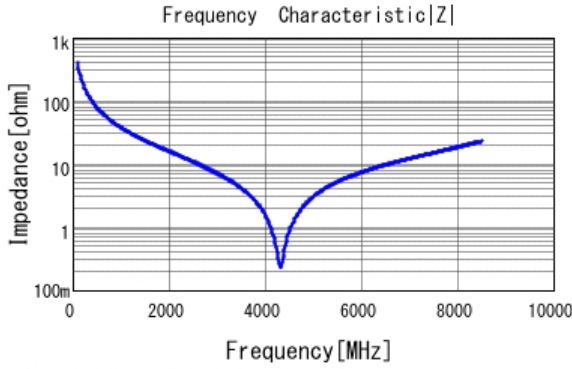
■ GJM1555C1H4R0BB01 |Z| DCOV, 25degC
