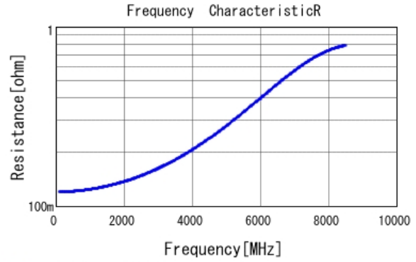
■ GJM1555C1H4R0BB01 R DCOV, 25degC
